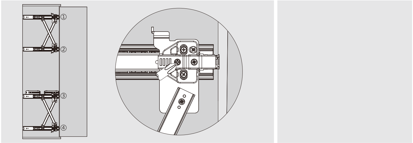
Adjust the screw No. 1 to make the door move inside Adjust the screw No. 2 to make the door move outside
